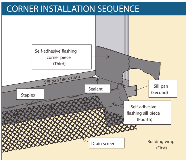
Multiple layers give redundant defense to water infiltration, while a sill pan returns any water within the installation back outside the wall.
