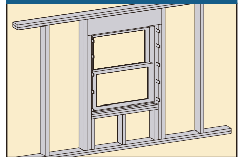
Shims are located uniformly and snugly between the window and the rough opening.
