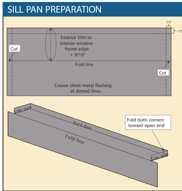
Multiple layers give redundant defense to water infiltration, while a sill pan returns any water within the installation back outside the wall.
